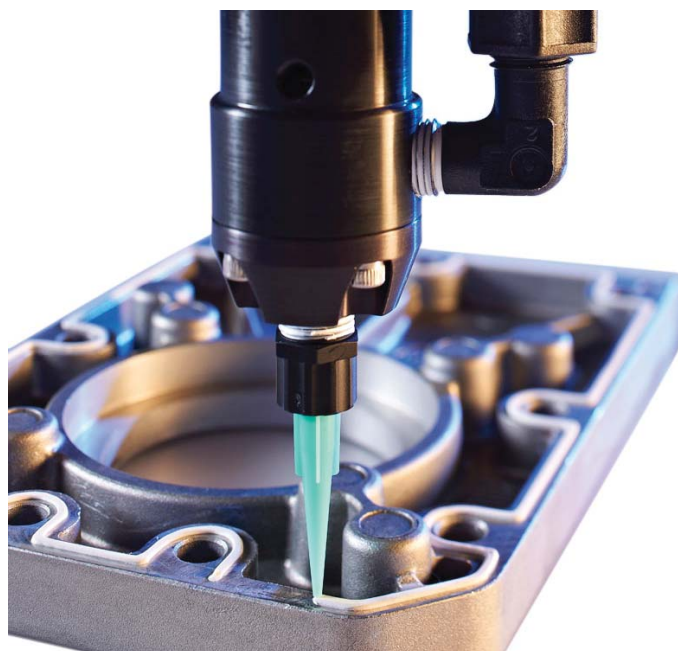
TS5322 - Gasketing
